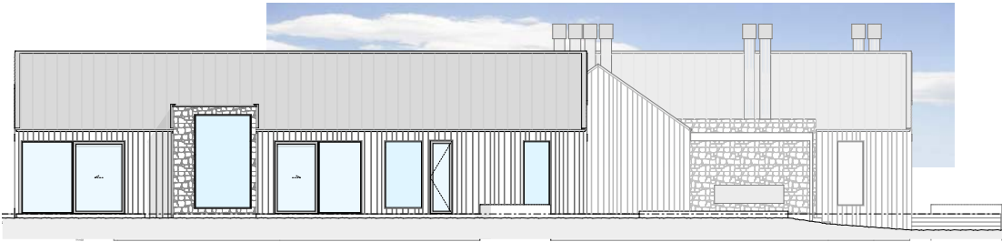
East Elevation
